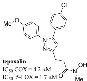
Fig. (7). Structure of tepoxalin.
