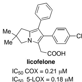
Fig. (13). Structure of pyrrolizine based COX/5-LOX dual inhibitor.
