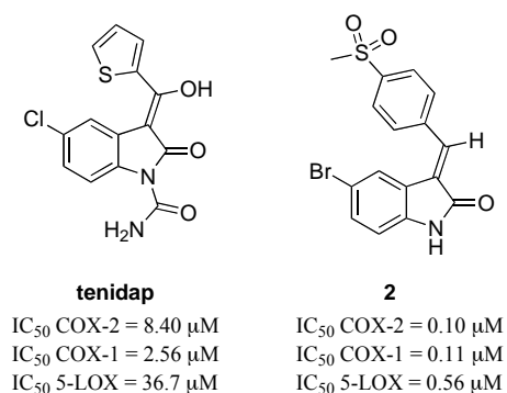
Fig. (11). Structures of NSAID based COX/5-LOX dual inhibitors.
