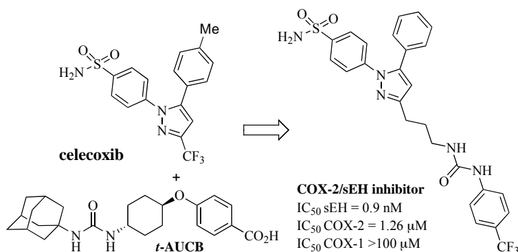
Fig. (14). Structure of COX-2/sEH dual inhibitor.
