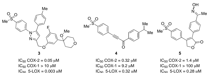
Fig. (12). Structures of coxib based COX-2/5-LOX dual inhibitors.
