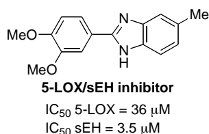
Fig. (15). Structure of 5-LOX/sEH dual inhibitor.
