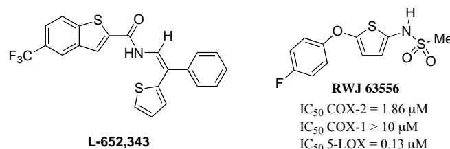
Fig. (8). Structures of thiophene based dual inhibitors.
