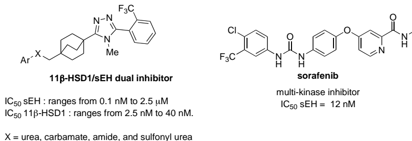
Fig. (18). Structures of 11 \beta -HSD1/sEH dual inhibitors and sorafenib.
