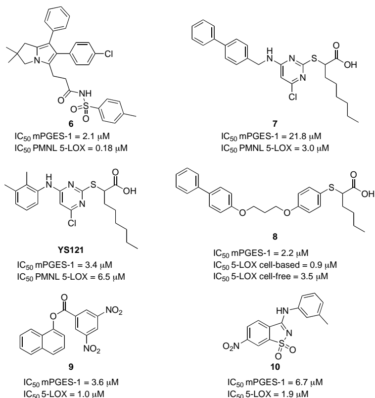
Fig. (16). Structures of 5-LOX/mPGES-1 dual inhibitors.
