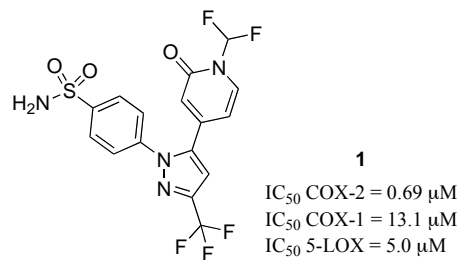
Fig. (9). Structure of pyridone based dual inhibitor.
