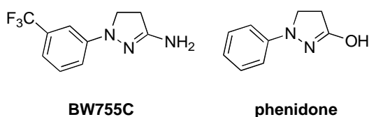
Fig. (6). Structures of pyrazoline derivatives.
