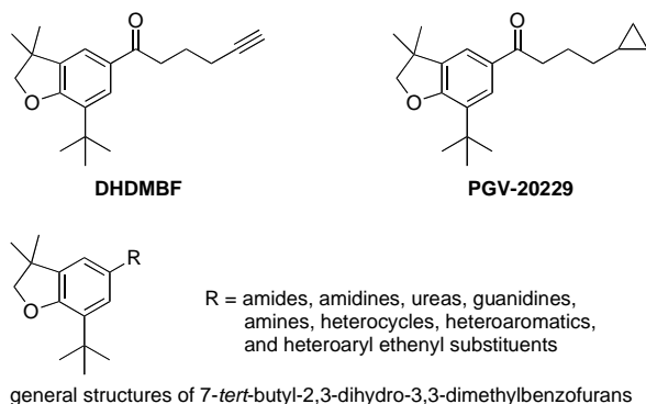
Fig. (10). Structures of DHDMBFs.
